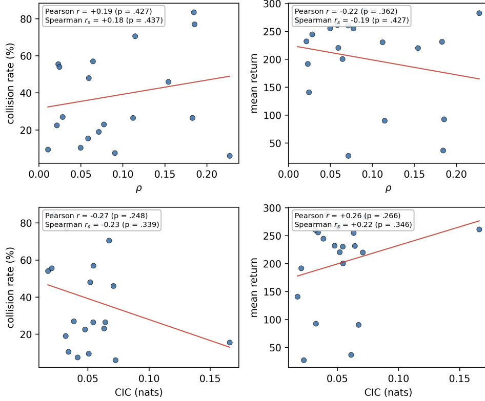
Figure 4.9: Seed-level relationships between the signalling metrics ( \rho , CIC) and task outcomes (collision rate, mean return) across 20 bimodal seeds. Each point is one seed and the line is an ordinary least-squares fit. Each panel is annotated with the Pearson r and the Spearman r_s over the 20 seeds, with the associated p -value. All four relationships are weak and none is significant. Exact values are given in Table B.5.
