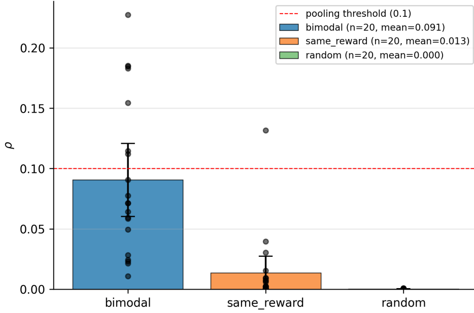
Figure 4.1: \rho by condition. Bars are means over the 20 seeds and error bars are 95% seed-level confidence intervals (Student- t over the seed means); points are individual seeds.
