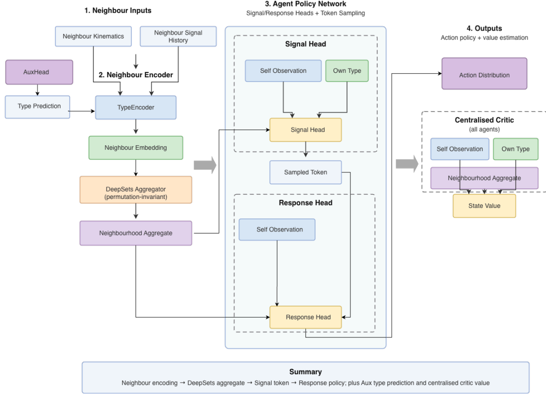
Figure 3.2: System architecture diagram. Neighbour kinematics and signal history pass through the shared TypeEncoder to produce a neighbour embedding, which the permutation-invariant DeepSets aggregator reduces to a neighbourhood aggregate. The Signal Head conditions on self-observation and own type to sample a token; the Response Head then conditions on self-observation, the neighbourhood aggregate, and that sampled token to produce the action distribution. The AuxHead supervises the neighbour embedding with a privileged type-prediction loss during training only, and is discarded at evaluation. The Centralised Critic pools all agents’ self-observations, types, and neighbourhood aggregates to estimate the joint state value
