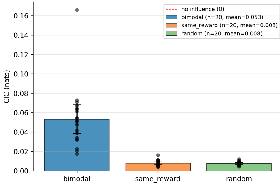
Figure 4.8: Causal Influence of Communication by condition (nats). Bars are means over the 20 seeds, error bars are 95% seed-level confidence intervals, and points are individual seeds.
