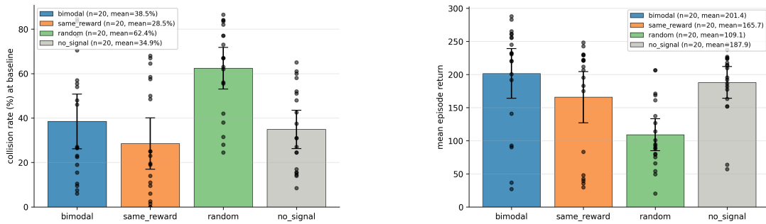
Figure 4.6: Collision rate and return by condition under the unmodified baseline. Left: the collision rate. Right: the mean episode return. Bars are means over the 20 seeds of each condition, error bars are 95% seed-level confidence intervals, and points are individual seeds.
