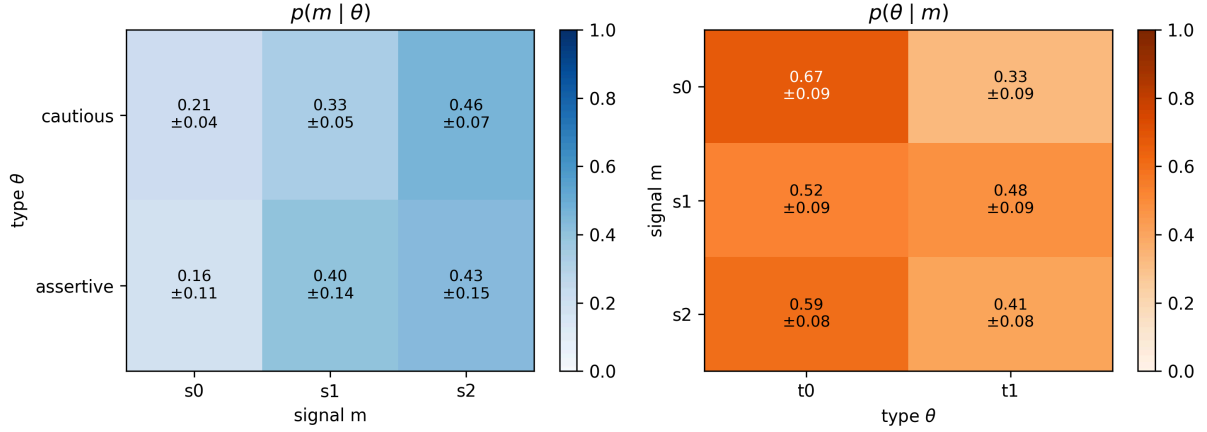
Figure 4.4: Signal use in the bimodal condition, mean over 20 seeds. (Left) p(m | \theta) , how each type distributes its tokens. (Right) p(\theta | m) , the type implied by a received token. The \pm values are 95% seed-level confidence intervals on each cell, computed as 1.96 standard errors over the 20 seeds.
