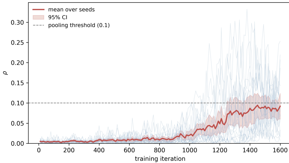
Figure 4.2: \rho over training for the bimodal condition. Faint lines are the 20 individual seeds; the solid line is the mean, and the shaded band is the 95% seed-level confidence interval at each logged iteration; the dashed line marks the pooling threshold \rho = 0.1 .
