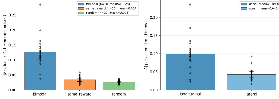
Figure 4.7: Counterfactual Decoding Effect across conditions. Left: change in the receiver’s mean action when the received token is altered with the scene frozen, by condition. Right: per-dimension change in the bimodal family. Bars are means over the 20 seeds, error bars are 95% seed-level confidence intervals, and points are individual seeds.
